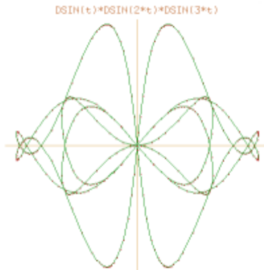
Figure 4.4: curve(\sin(t) * \sin(2 * t) * \sin(3 * t), \sin(4 * t) * \sin(5 * t) * \sin(6 * t)), t = 0..2 * \pi
